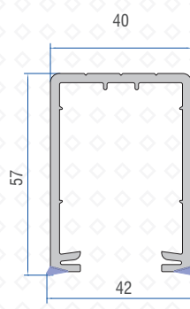
Stiffener Profile / Hurricane Bar Profile 40201-11000
