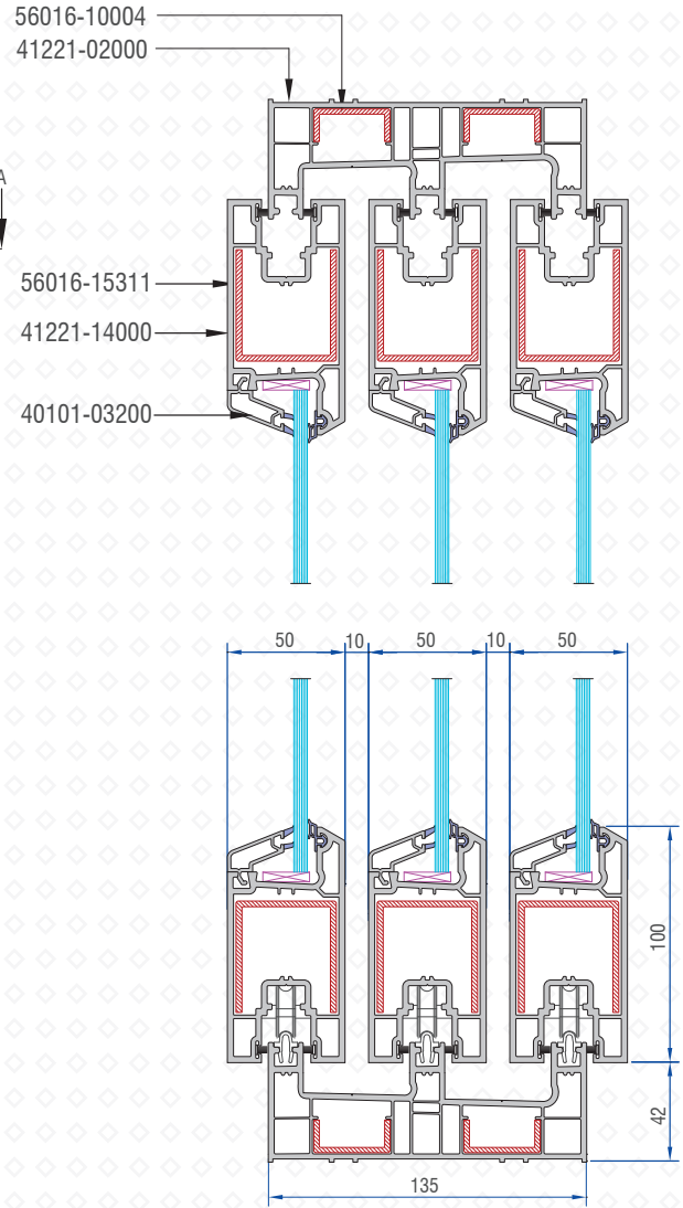
SEC B-B
