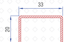
65mm Sash Reinforcement 1.5mm : 56016-15117
