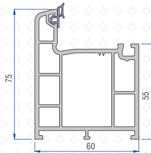
Super Frame Profile 41101-19000
