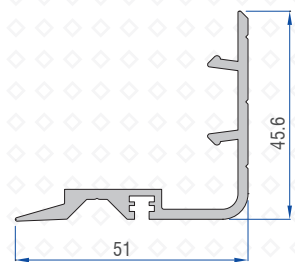
Mega Sash Cover Profile 41201-06300
