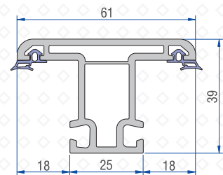
Mullion Profile 41201-04000
