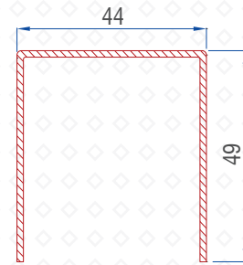
Mega Sash Reinf. 1.5mm : 56016-15311
