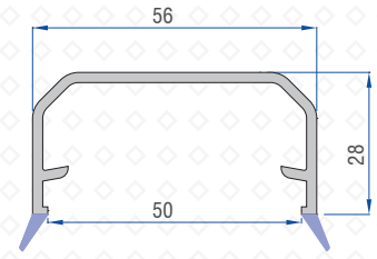
Hurricane Bar Profile 40201-01000
