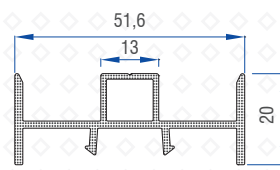
Inline Sash Adaptor (I-64) 50502-11065
