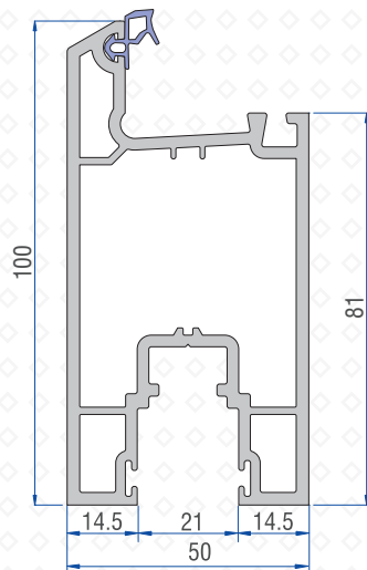
Mega Sash Profile (I-75) 41221-14000
