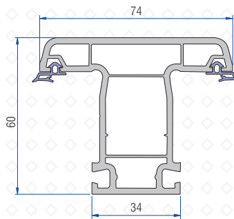
Mullion Profile 41101-12000
