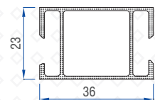
Multi Track Adaptor (Alm) 50502-11017
