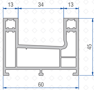
Double Rail Profile 41201-12000
