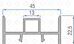
Inline Sash Adaptor (Alm) 50502-11060
