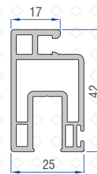
Screen Sash Profile 41301-05200
