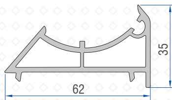
Bay Pole Adaptor 2108 - 3104
