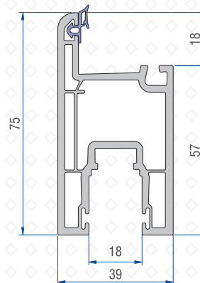
Super Sash Profile 41201-03000
