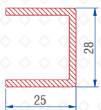
Super Sash Reinf. 1.5mm : 56016-15017
