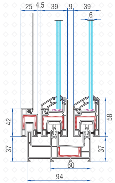
SEC B-B
