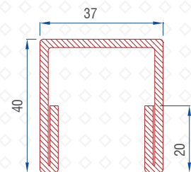
Mega Sash Reinf. 1.5 mm : 56016-15147
