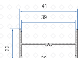
Adaptor for Super Screen Sash (New) 50502-11078
