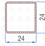
Grill Reinf. (New) 1.0mm : 56016-10044
