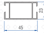
Multi track Adaptor (Alm) 50502-11031
