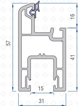
Sash Profile 40502-13000
