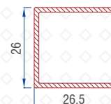
Mega Sash Reinf. (Secondary) 1.5mm : 56016-15057
