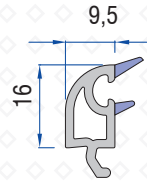
Single Glazing Bead 40502-14000
