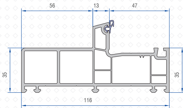
Frame with Grill & Mesh 41101-16100
