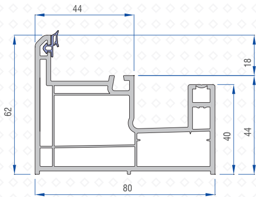
Mono Rail Profile 41164-10400
