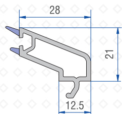
Single Glazing Bead (6mm) 40101-03200
