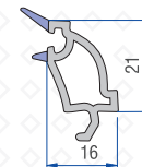
Double Glazing Bead (24mm) 40101-03500
