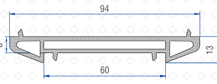
Casement - Sliding Profile Middle Coupler (Alm) 50502-11040
