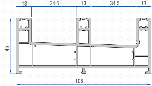
Triple Rail Profile 41201-15000
