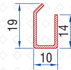
Adaptor Screen Sash Reinf. 1.2mm : 56016-12041
