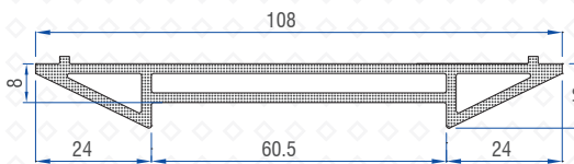
New 3-Track Coupler (Alm) 50502-11057
