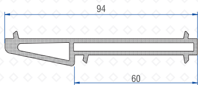
Casement - Sliding Profile Coupler (Alm) 50502-11039
