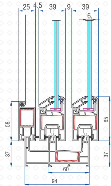
SEC B-B
