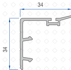
Sash Cover Profile 40502-13100
