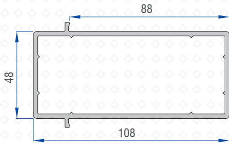
LARGE COUPLING PROFILE** 41165-30100G
