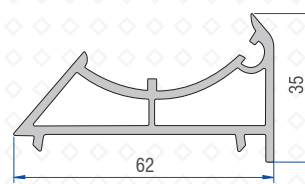
Bay Pole Adaptor / Pipe Adaptor Profile 2108-3104
