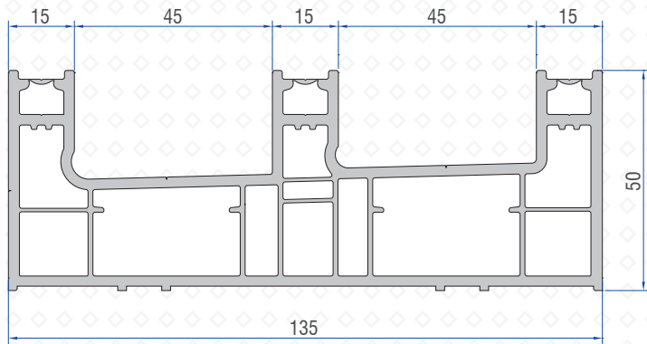
Triple Rail Profile 41221-02000
