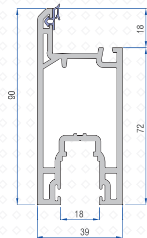
Mega Sash Profile 41201-07000
