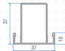
Super Screen Sash Mullion-3T 50502-11077
