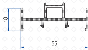
Inline Sash Adaptor (Alm) 50502-11035
