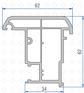
Lap Joint Profile 41101-15000
