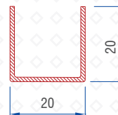
Screen Sash Reinf. 1.5mm : 56016-15501
