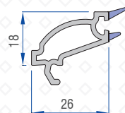
Single Glazing Bead (6mm) 41064-30100
