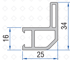
Screen Sash Adaptor 41301-05100
