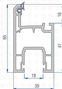
65mm Sash Profile 41201-03200
