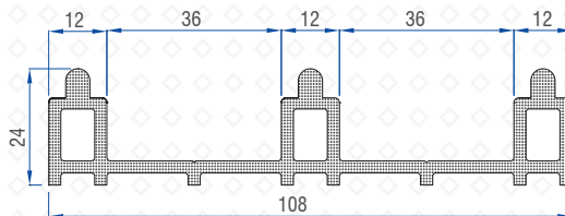
3-Track Low Threshold (Alm) 50502-11047
