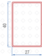
Super Frame Reinf. 1.0mm : 56016-10056
