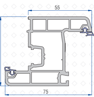
Inward Opening Sash Profile 41101-13100
