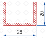
Frame / Mullion Reinf. 1.0mm : 56016-10002
