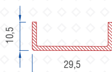
2T/2.5T Frame Reinf. 56016-10007
