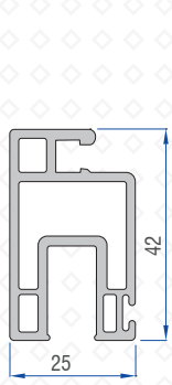
Screen Sash Profile 41301-05200
