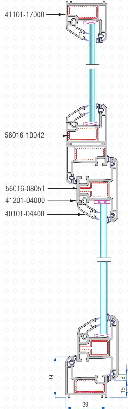
SEC B-B
