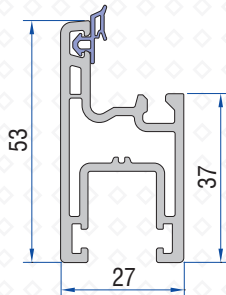
Sliding Sash 41231-13100
