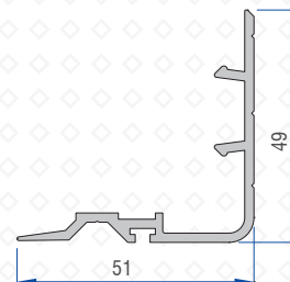
Mega Sash Cover Profile 41064-40300
