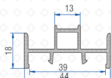
Inline Sash Adaptor (Alm) 50502-11034
