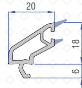
Single Glazing Bead (6mm) 40101-04400
