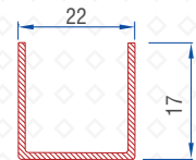
Sash Reinf. 1.0mm : 56016-10073
