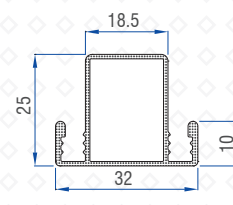
Mega Screen Sash Mullion-2.5T (Alm) 50502-11058
