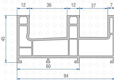
Double Rail with Screen Track Profile 41201-05100
