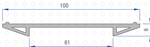
Casement Sliding Middle Coupler 2.5T (I-64) 50502-11063
