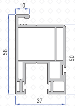
Super screen sash (New) 41221-03000
