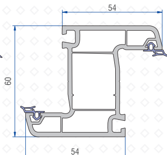
Outward Opening Mullion Profile 41101-12100
