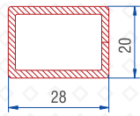
Frame / Mullion Reinf. 1.0mm : 56016-10001
