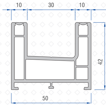
Double Rail Profile 40502-11000
