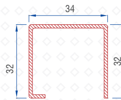
Super Sash Reinf. 1.5 mm : 56016-15137
