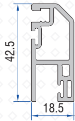
Adaptor Screen Sash 41301-05000
