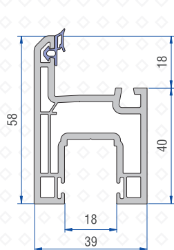
Sash Profile 41201-03300
