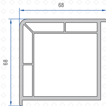
Corner Profile (90°) 2108-3101
