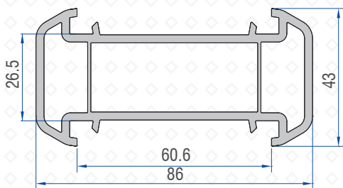
LARGE COUPLING PROFILE 40107 - 01200
