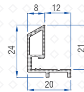
Mesh Adaptor (Alm) 50502-11055
