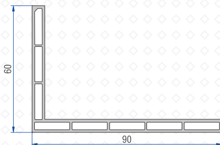
Border Profile 40110-02000
