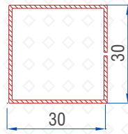
Double Rail Reinf. 1.0mm : 56016-10301
