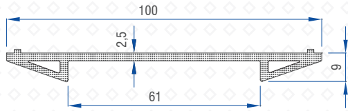
Casement Sliding Middle Coupler 2.5T (I-64) 50502 - 11063
