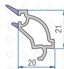
Double Glazing Bead (20mm) 40101-03400
