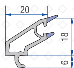
Single Glazing Bead (6mm) 40101-04400
