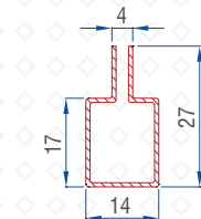
Sash/ Mullion Reinf. 56016-08051
