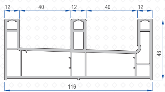
Triple Rail Profile 41264-10300
