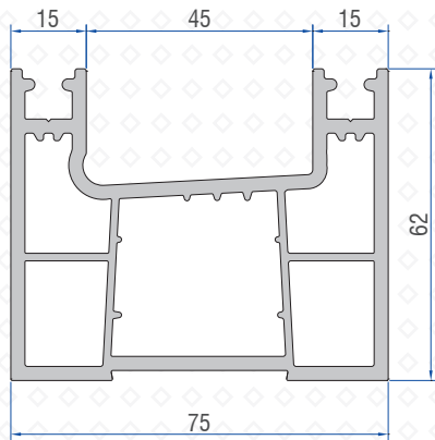
Double Rail Profile 41221-01000
