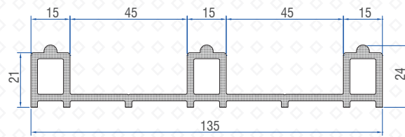
3-Track Low Threshold (I-75) Alm 50502-11069
