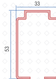
Stiffener Profile / Hurricane Bar Reinf. 2.0mm : 56016-20072
