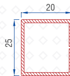
Mega Screen Sash Reinf. / Super Screen Sash 1.5mm : 56016-15601
