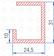
Window Sash Reinf. 1.5mm : 56016-15011
