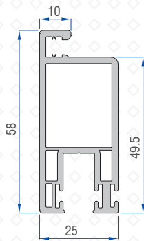
Mega Screen Sash Profile 41201-05300
