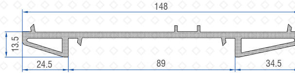
Coupler for Mesh and Grill Frame (Alm) 50502-11046
