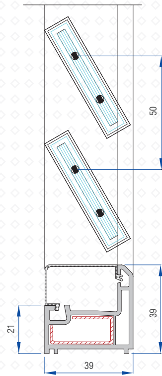
SEC B-B
