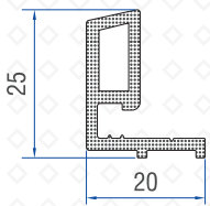
Mesh Adaptor (Alm) 50502-11041
