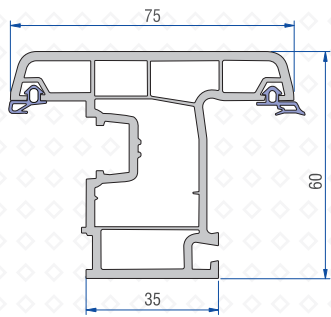
Window Sash Profile 41101-13000
