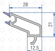
Single Glazing Bead (12mm) 40101-03200
