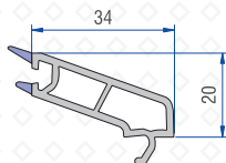
Single Glazing Bead (6mm) 40101-03300
